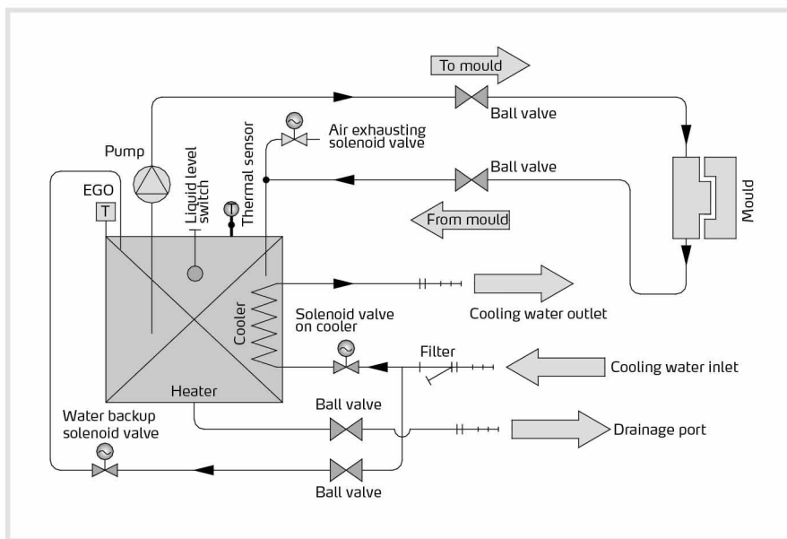
System Flow (Indirect Cooling)
